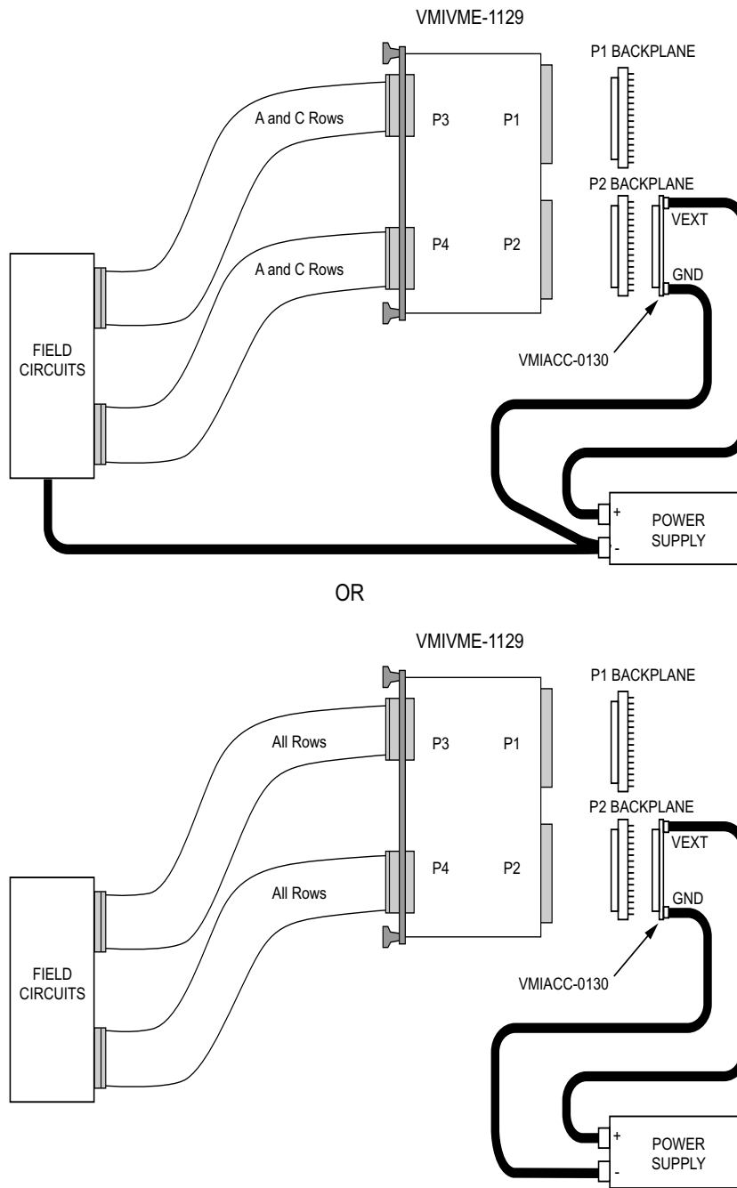
Figure 1. P2 External Power Connections
