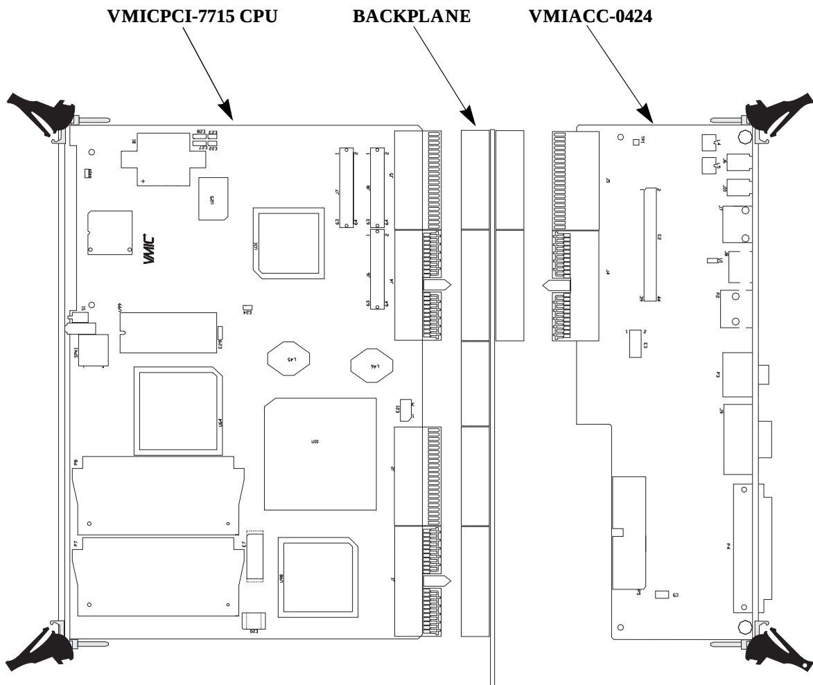
Figure 1-2 Installation of the VMIACC-0424 Adapter Board with a VMICPCI-7715
