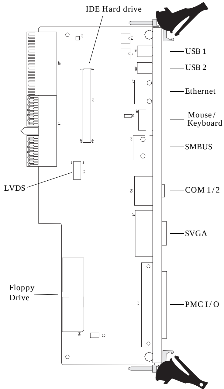
Figure 1-1 VMIACC-0424 CompactPCI Rear Transition Utility Board
