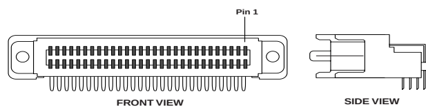
Figure 1-14 P4 PMC I/O Connector
