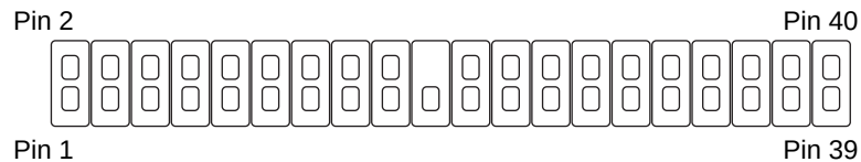
Figure 1-3 E2 40-pin IDE Header
