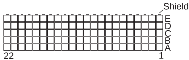
Figure 1-7 CompactPCI Connector (J5)
