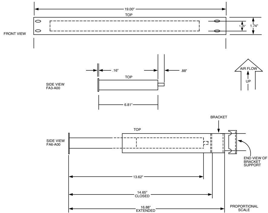
Figure 1. Front and Right Side Outline Dimensions of Rack Mountable Fan Assembly
