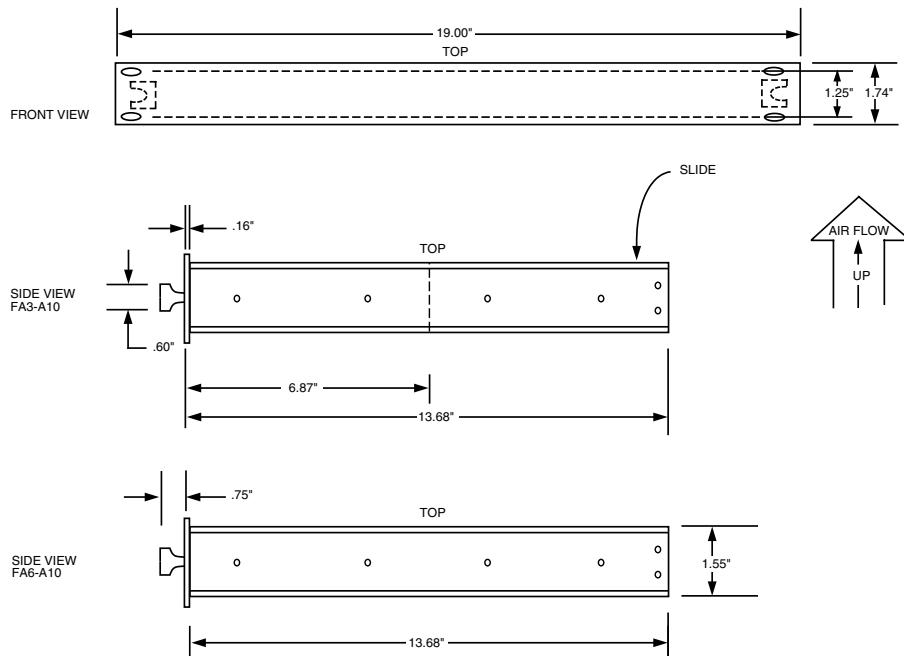
Figure 2. Front and Right Side Outline Dimensions of Slide Mounted Fan Assembly
