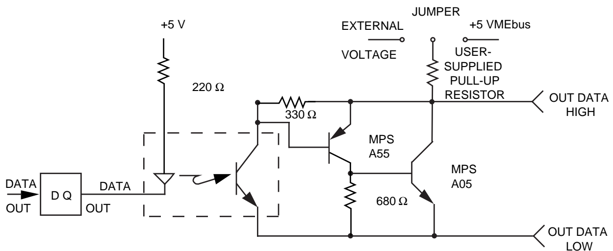
Figure 4. Typical Output Configuration
