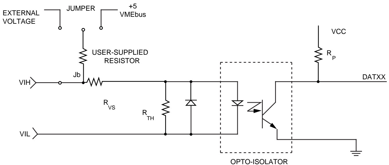
Figure 2. User Input Connection Circuit
