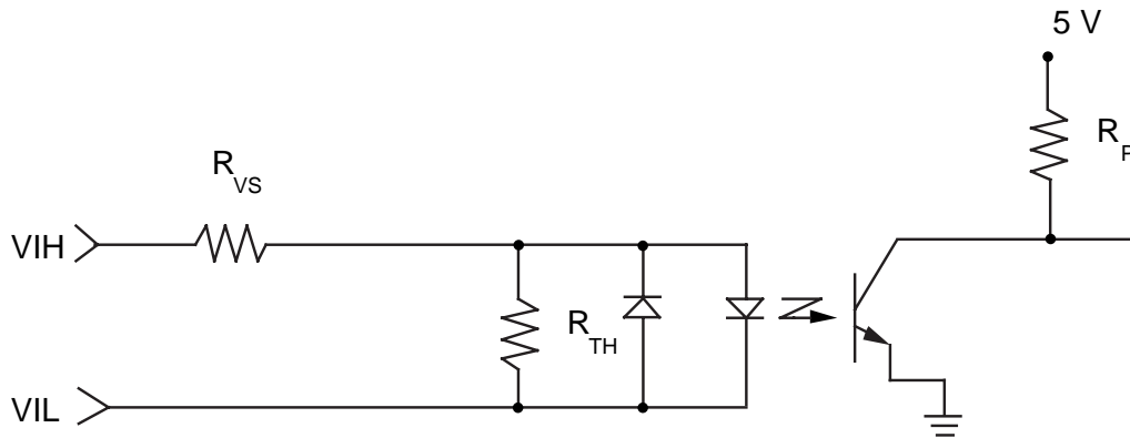
b. TYPICAL VOLTAGE SENSE OPTO INPUT
