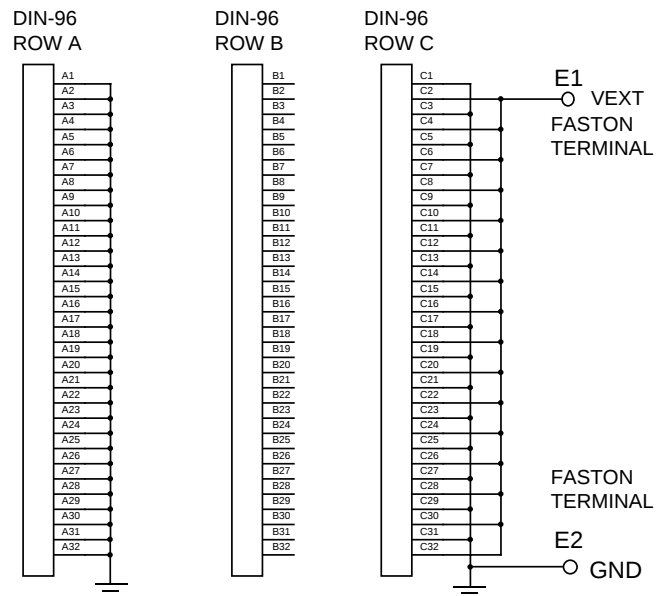
VMIACC-0129 Schematic
