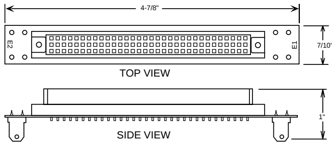
VMIACC-0129 Physical Dimensions
