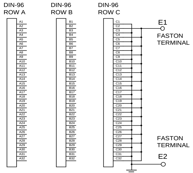
VMIACC-0130 Schematic
