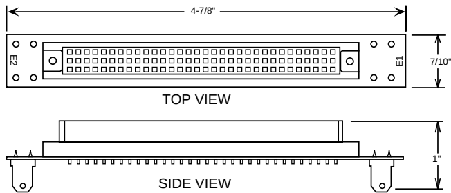
VMIACC-0130 Physical Dimensions
