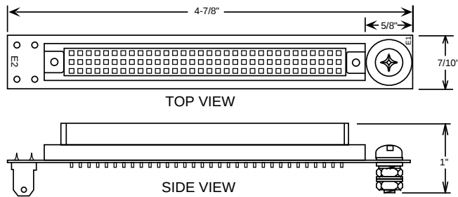
VMIACC-0131 Physical Dimensions
