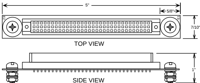
VMIACC-0132 Physical Dimensions
