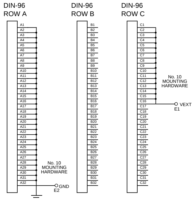
VMIACC-0132 Schematic
