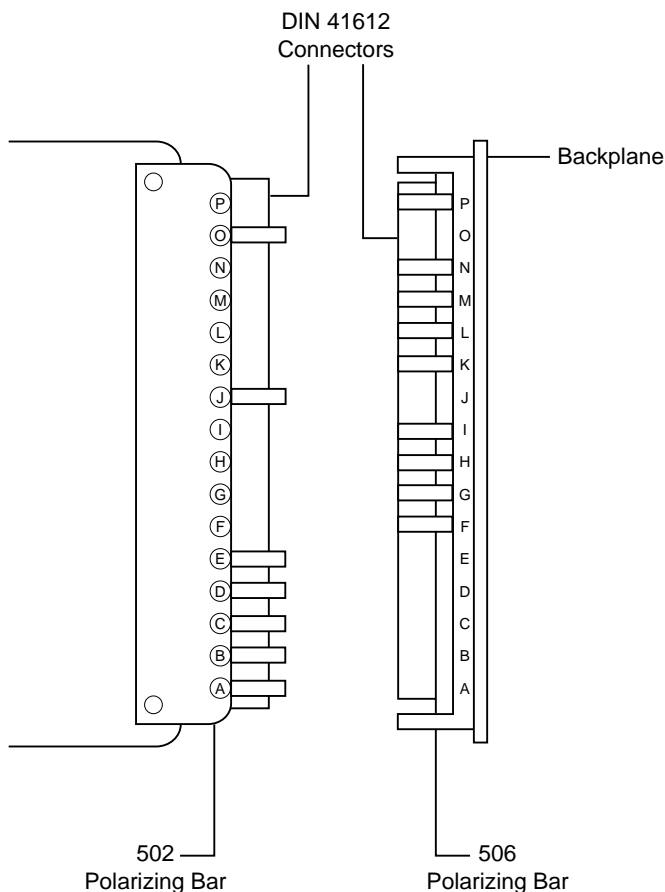
Figure 1. 502 and 506 Polarizing Bars
