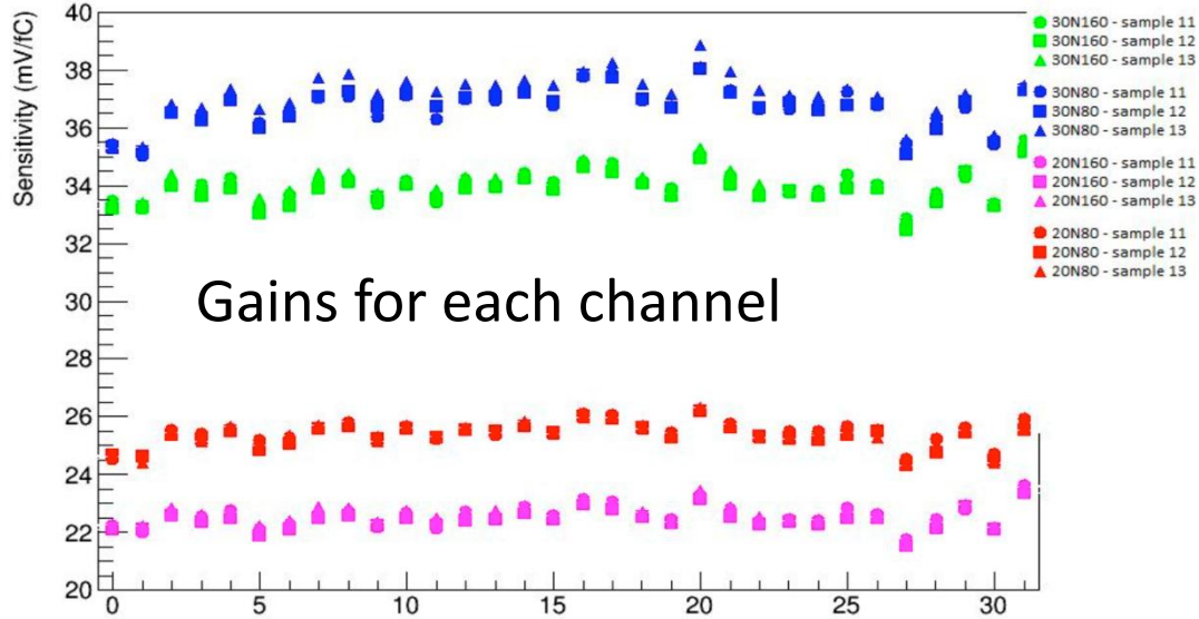
Mean sensitivity for samples 11, 12 and 13
