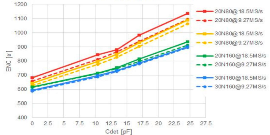
Average Noise vs. Cdet
