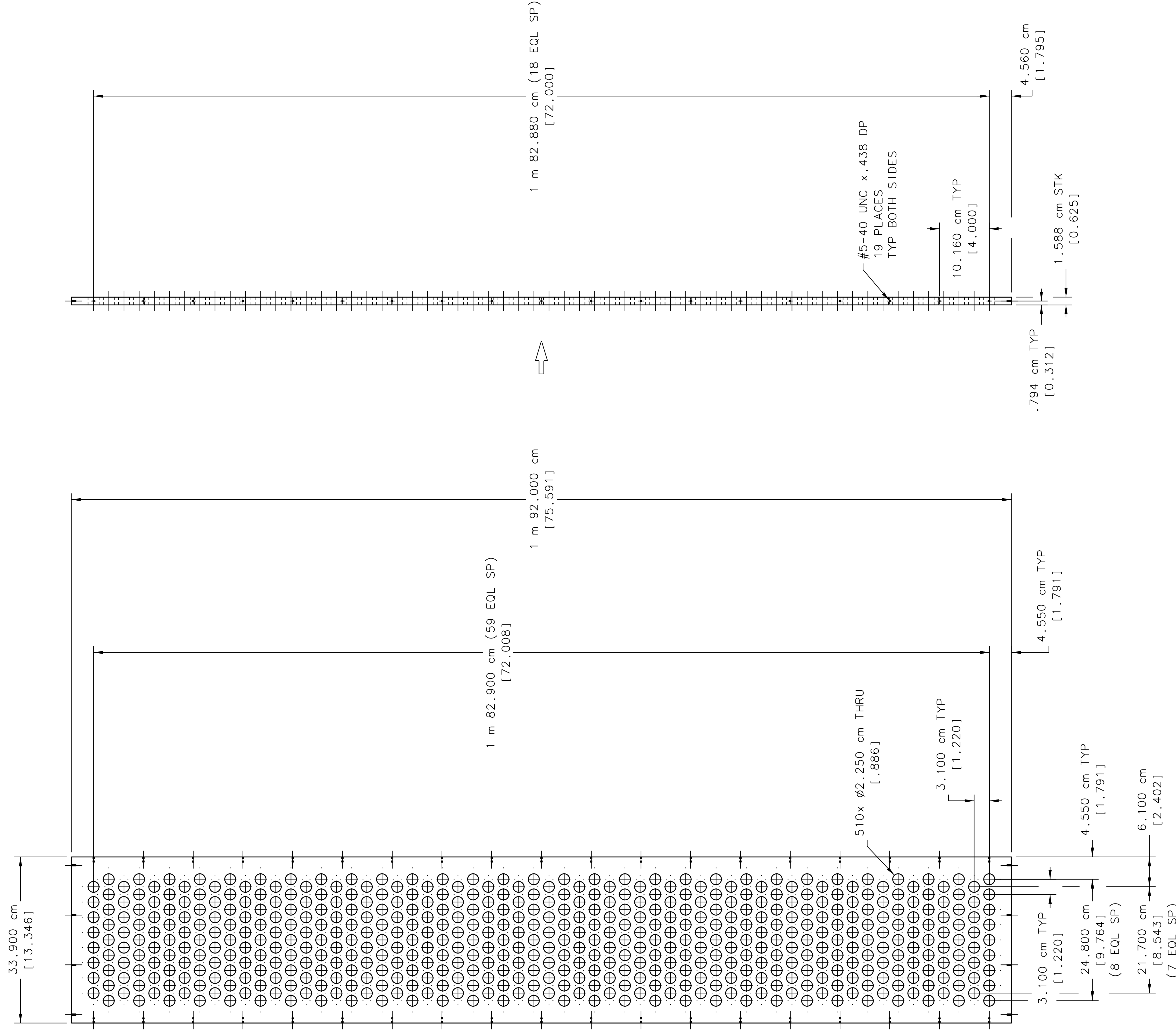
FRONT VIEW 1-7A
