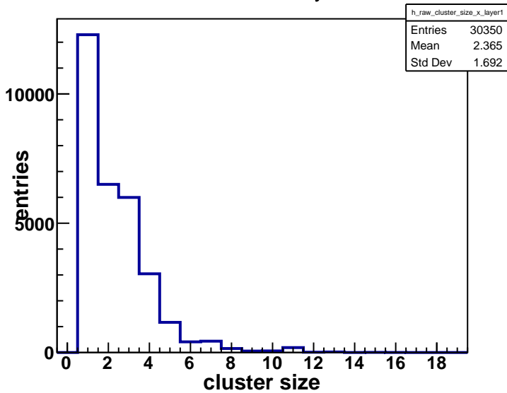
x cluster size layer1
