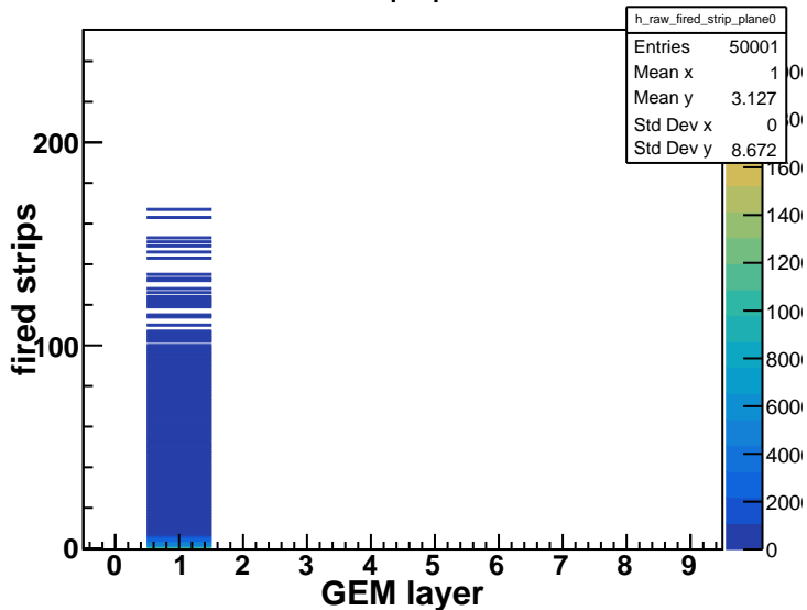
fired strips plane0
