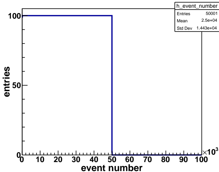
event number
