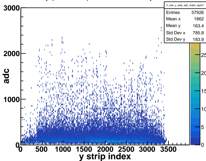
y plane strip adc vs index layer1
