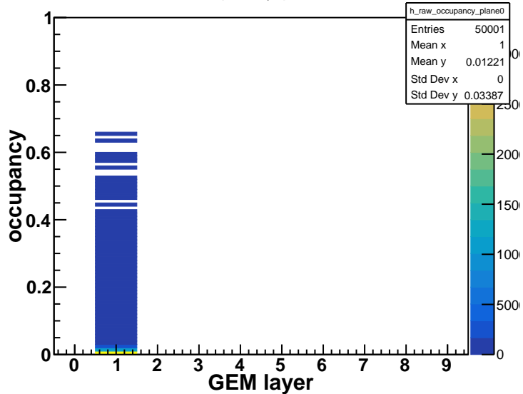
occupancy plane0
