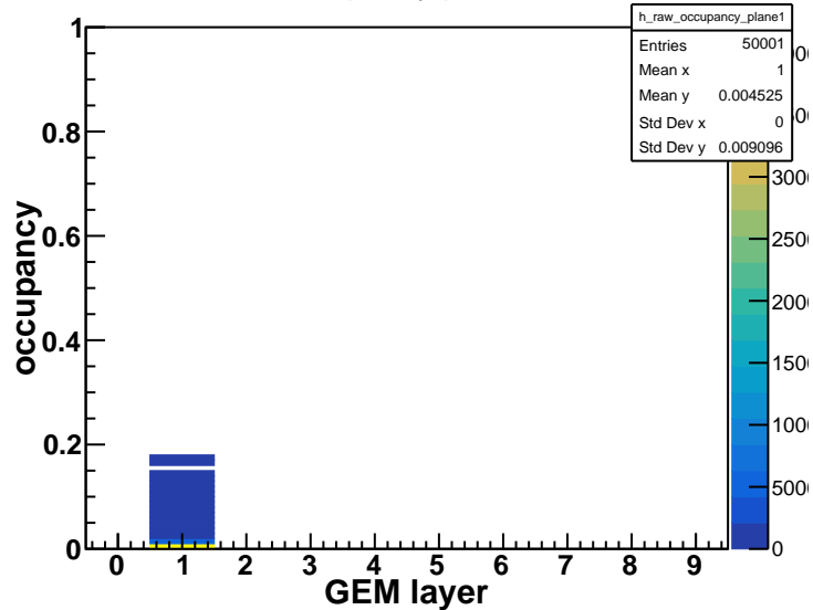
occupancy plane1
