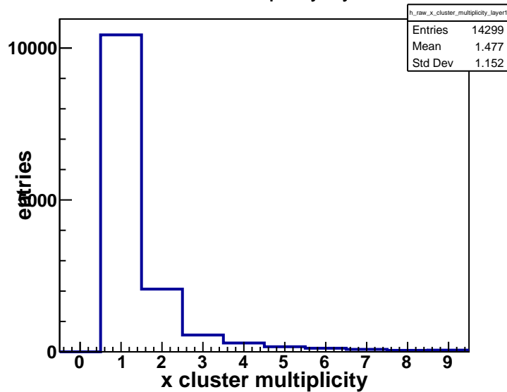
x cluster multiplicity layer 1
