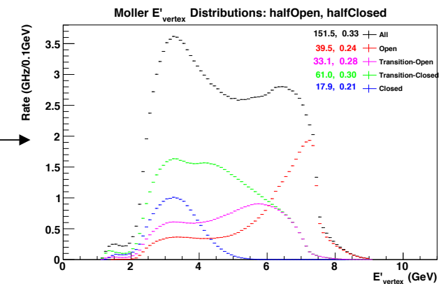
← HalfOpen/HalfClosed
