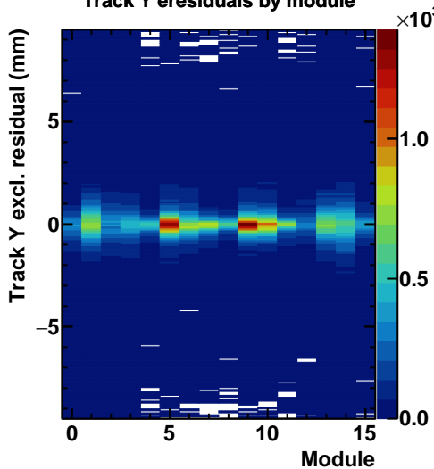
Track Y residuals by module
