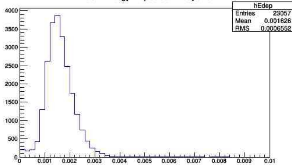
Muon Energy Deposition - Layer 3
