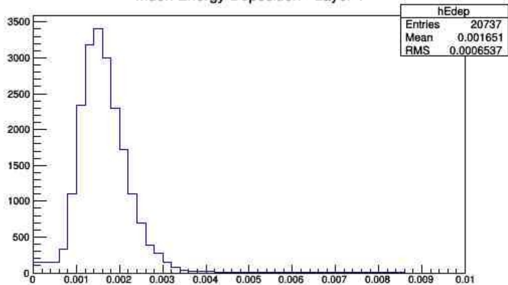
Muon Energy Deposition - Layer 1
