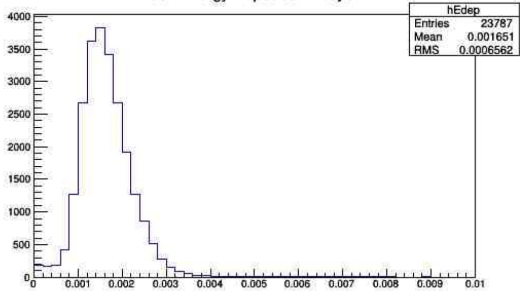
Muon Energy Deposition - Layer 2
