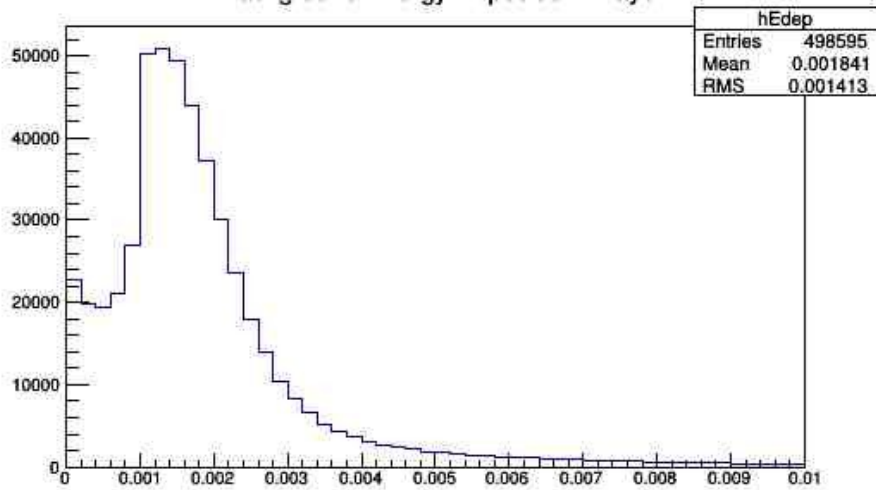
Pi- Background Energy Deposition - Layer 2
