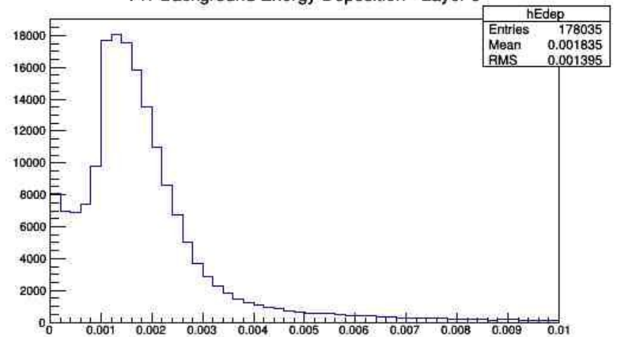
Pi+ Background Energy Deposition - Layer 3
