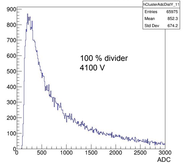
Y axis cluster charge_11
