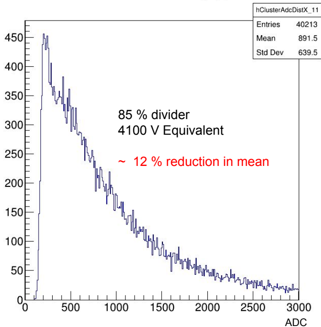
X axis cluster charge_11
