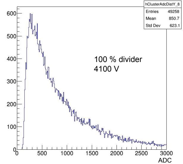
Y axis cluster charge_8
