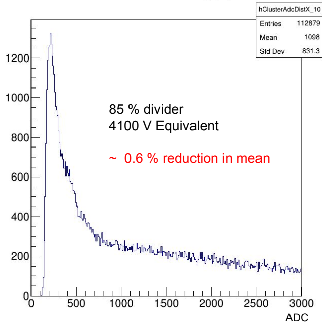
X axis cluster charge_10
