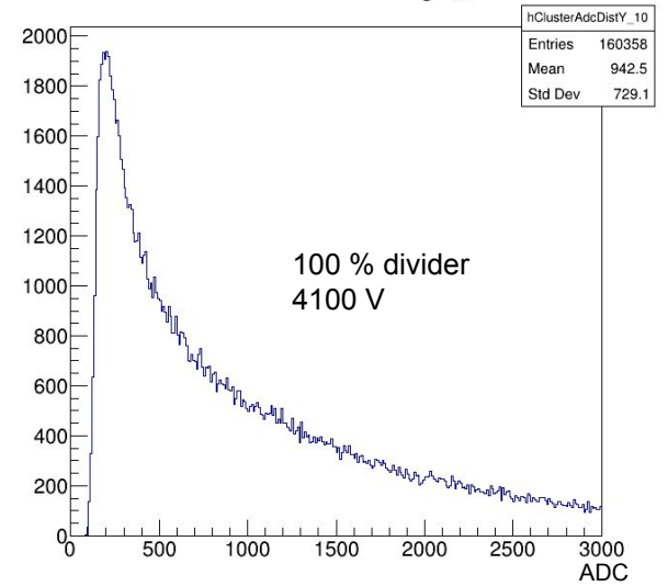
Y axis cluster charge_10
