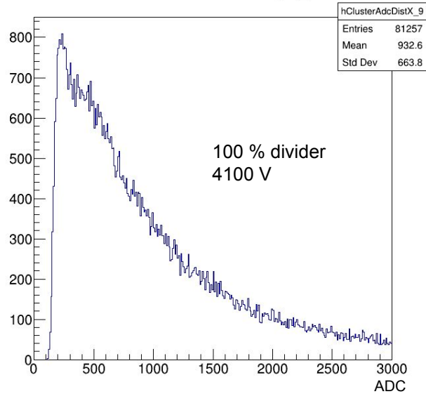
X axis cluster charge_9
