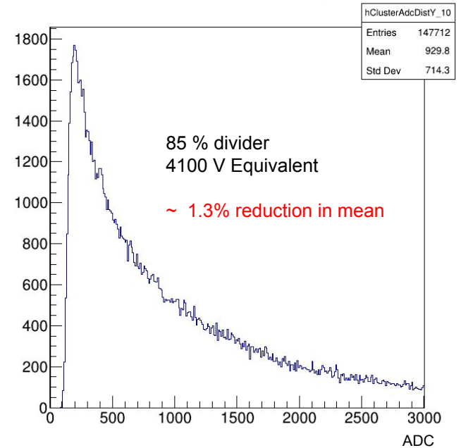
Y axis cluster charge_10
