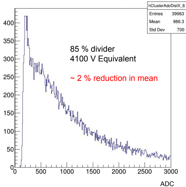
X axis cluster charge_8
