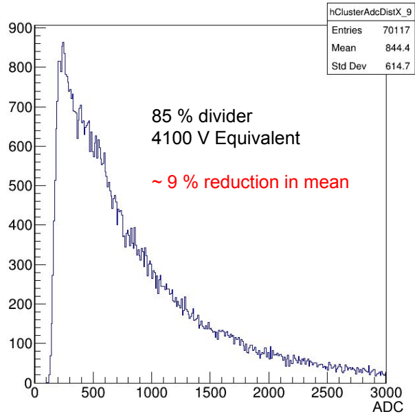
X axis cluster charge_9
