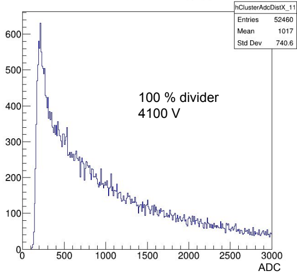
X axis cluster charge_11
