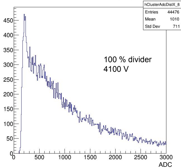
X axis cluster charge_8
