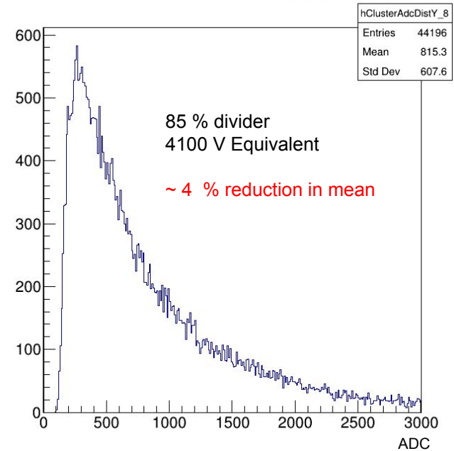
Y axis cluster charge_8
