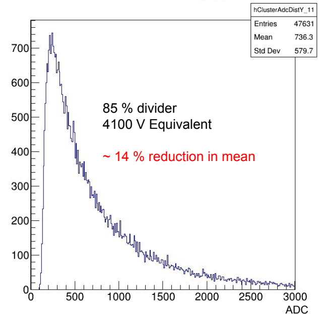
Y axis cluster charge_11
