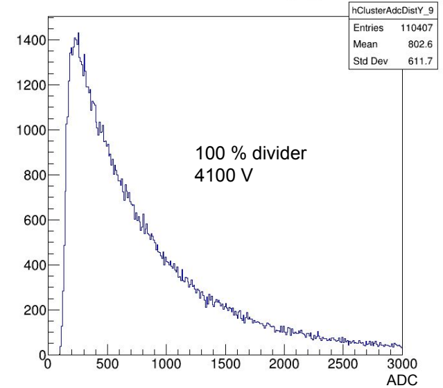
Y axis cluster charge_9
