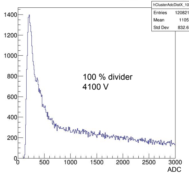
X axis cluster charge_10
