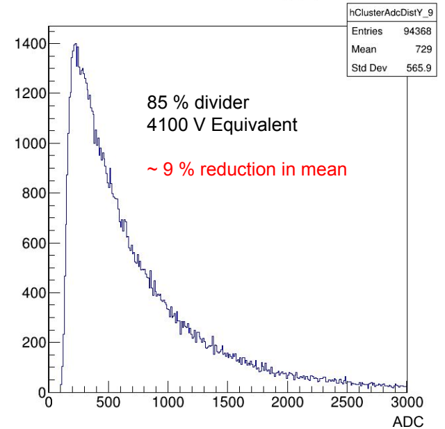
Y axis cluster charge_9
