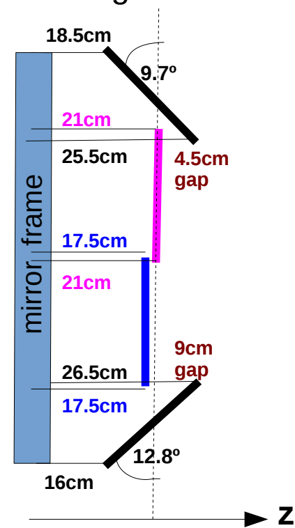
Right view
