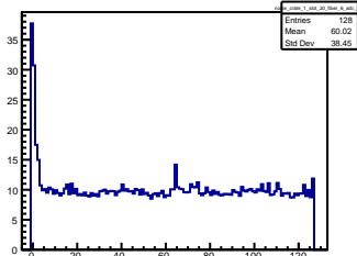
noise_crate_1_slot_20_fiber_6_adc_8
