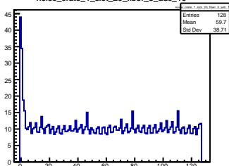
noise_crate_1_slot_20_fiber_3_adc_10
