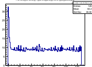
noise_crate_1_slot_20_fiber_5_adc_6
