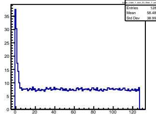
noise_crate_1_slot_20_fiber_7_adc_7
