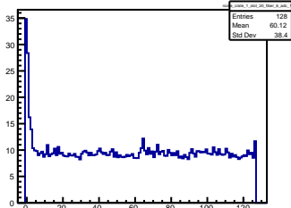
noise_crate_1_slot_20_fiber_6_adc_12
