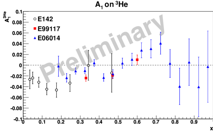
Figure 10: Preliminary E06-014 measurement of A_1^{^3\text{He}} at 4.74 GeV, compared to ^3\text{He} data from E142 at SLAC [21] and E99-117 in Hall A [10] [2].
