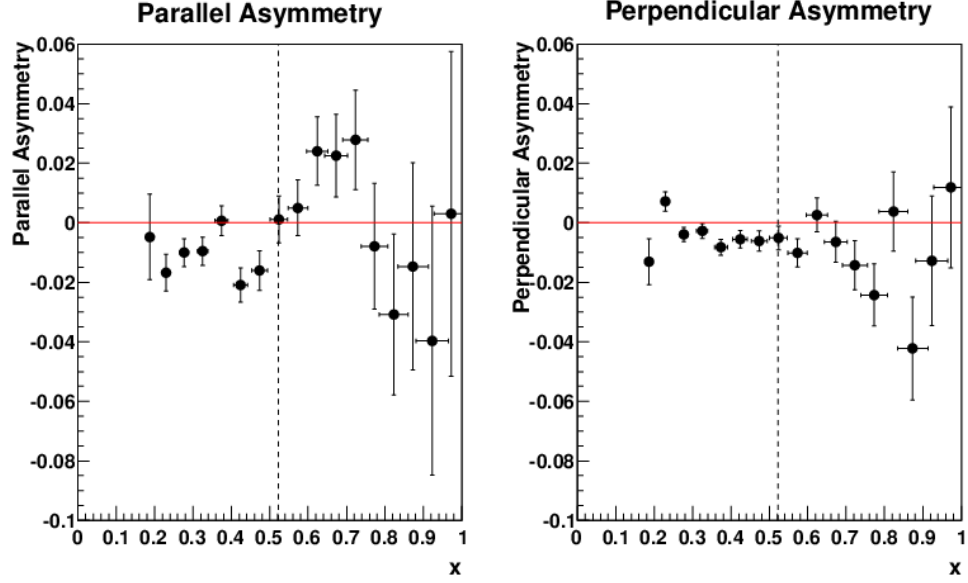
Figure 9: A_{\parallel} and A_{\perp} on ^3\text{He} are plotted vs x at a beam energy of 4.74 GeV. The dashed line is W = 2 GeV [2].
