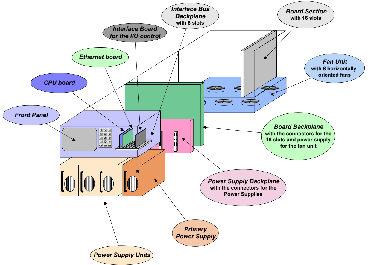
Fig. 3.1 – Details of the mechanical parts contained in the SY1527 mainframe
