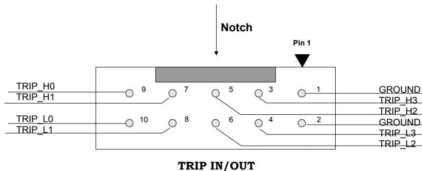
Fig. 4.1 – TRIP IN/OUT pin assignment
