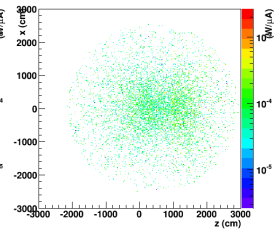
Bottom Disk. Det: Neutron from All Area
