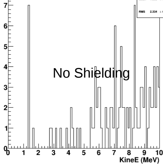
Neutron from Col-3 Area in KE<10 MeV Range
