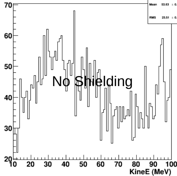
Neutron from Col-3 Area in 10<KE<100 MeV Range
