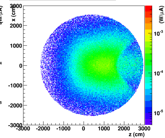
Bottom Disk. Det: \gamma from All Area
