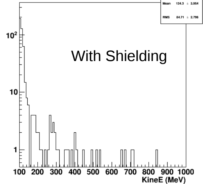
Neutron from Col-3 Area in 100<KE MeV Range
