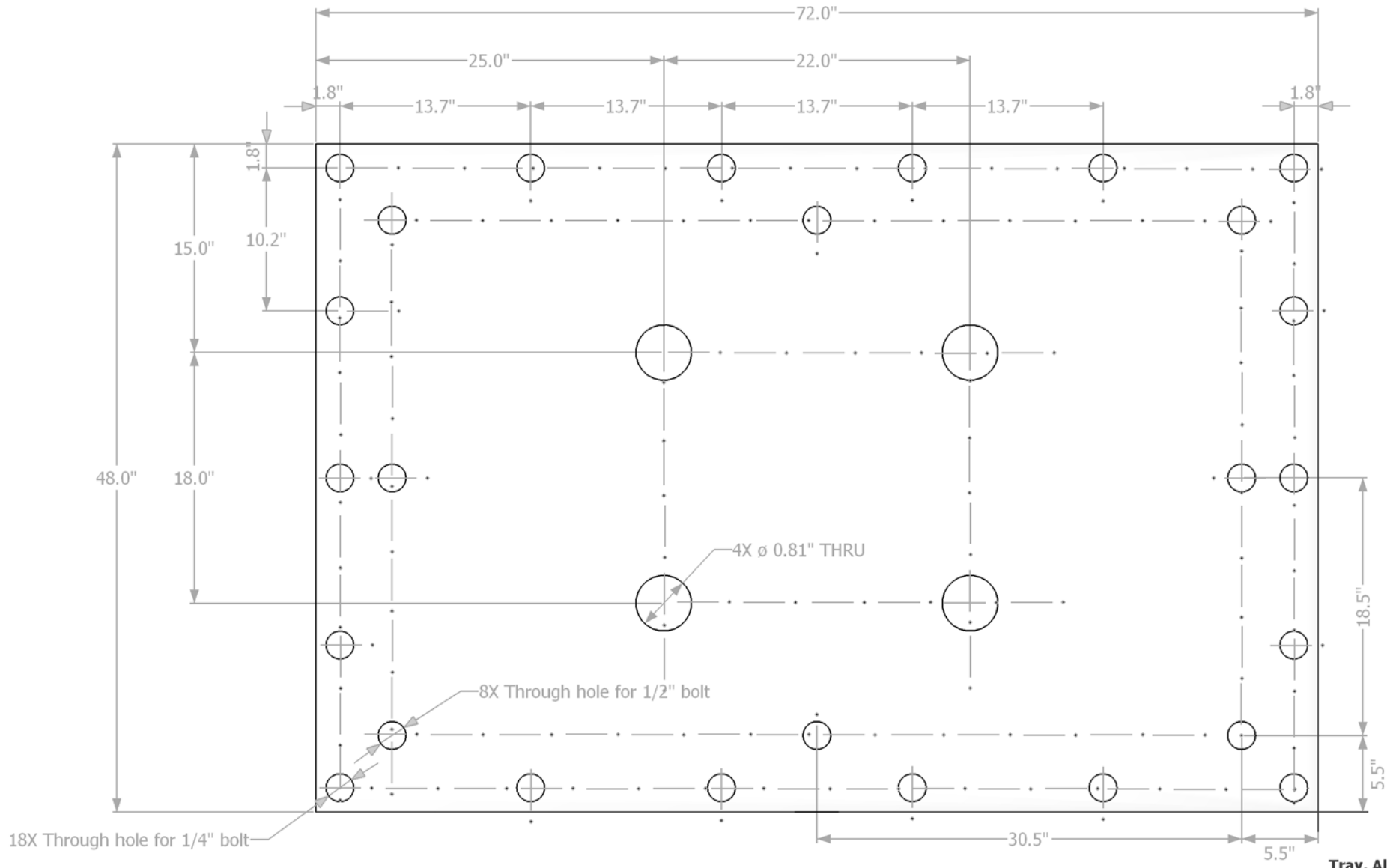
Tray, Al thickness=0.5" Top View Huan Yao #5007 04/25/2018
