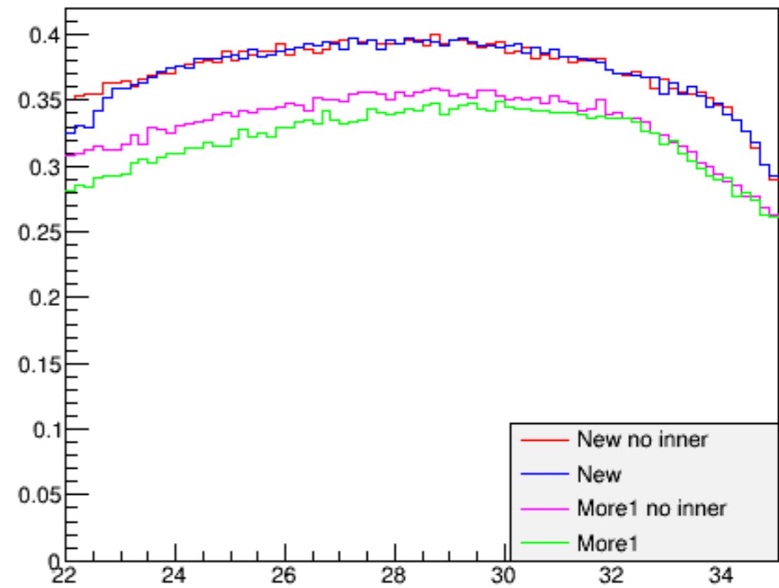
Acceptance vs theta
