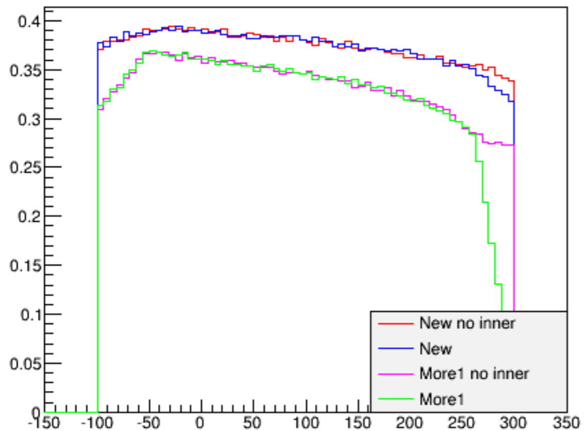
Acceptance vs z_v
