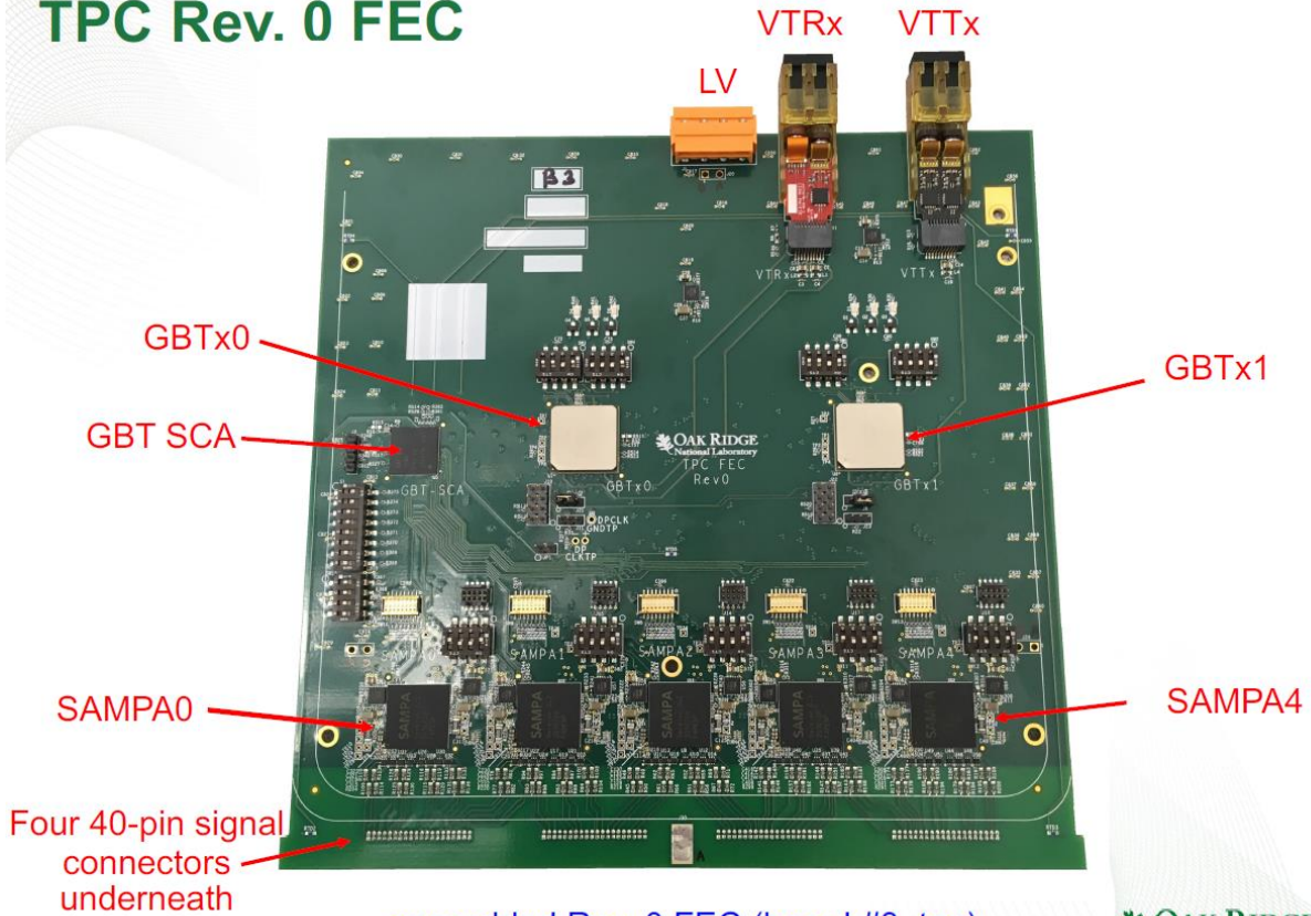
assembled Rev. 0 FEC (board #3, top)
