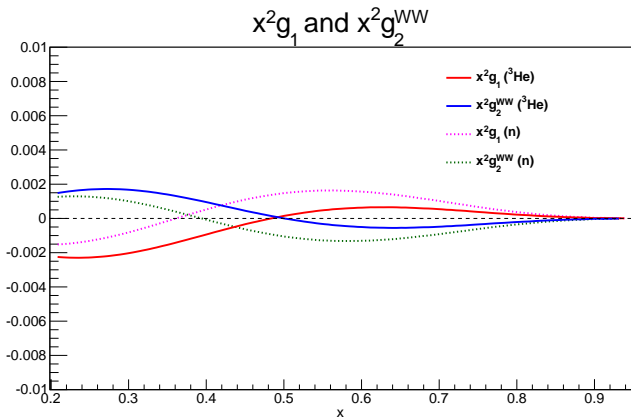
Figure: Plot shows the DSSV results for {}^3\text{He} and neutron g_1 and g_2^{WW} structure functions at E06-014 5.89 GeV kinematics.
