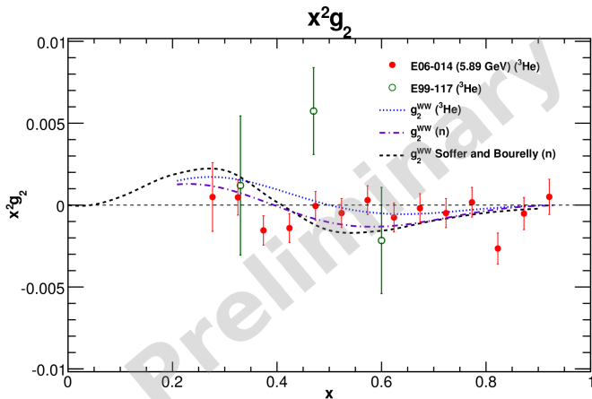
Figure: E06-014 preliminary ^3\text{He} g_2 compared to DSSV fit, Soffer and Bourelly fit and E99-117 data.
