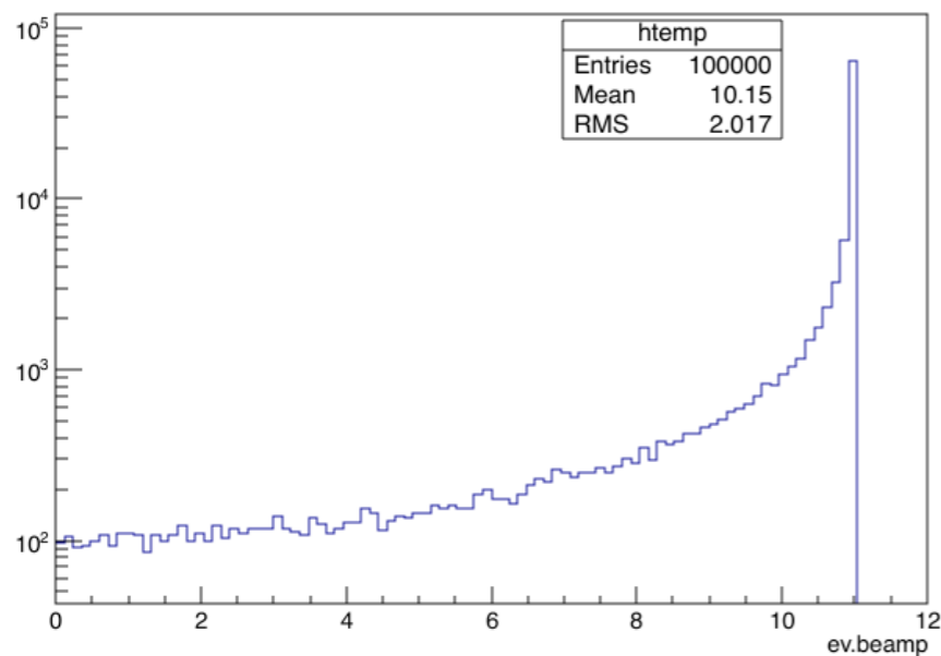
ev.beamp
