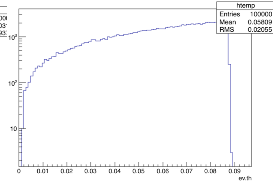
ev.th
